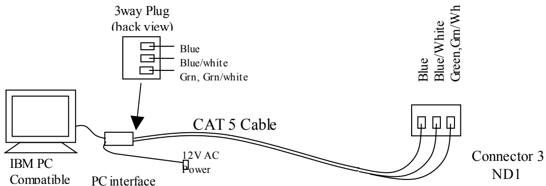
Connection of PC interface to the ND1 controller
